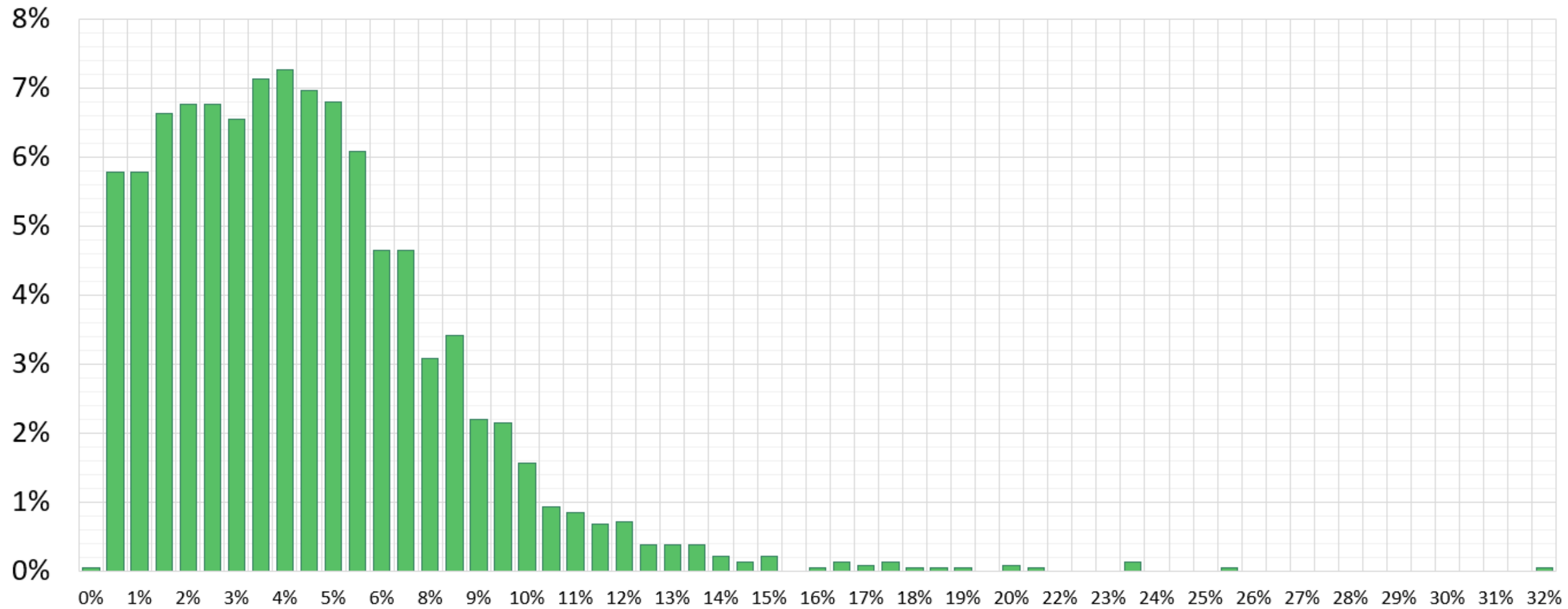
Percentage for Positive RTN ($SPY, 39D)
