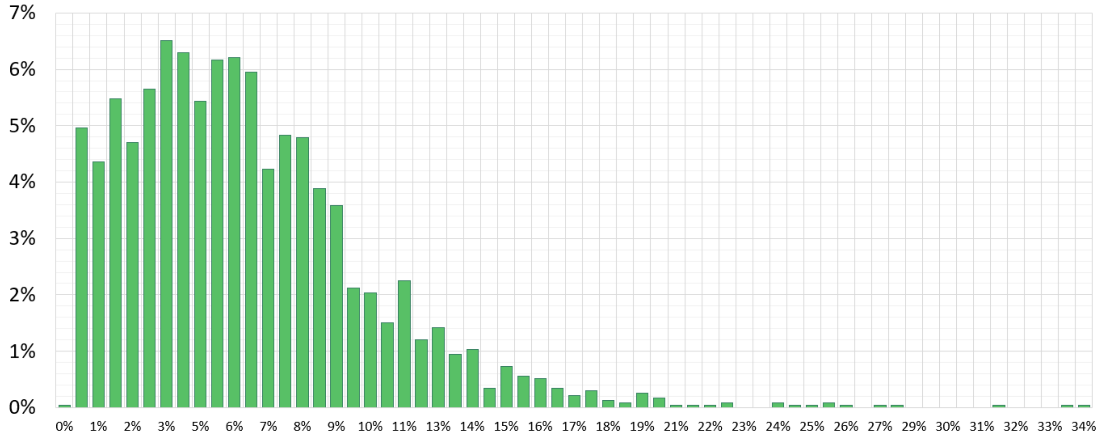
Percentage for Positive RTN ($QQQ, 39D)
