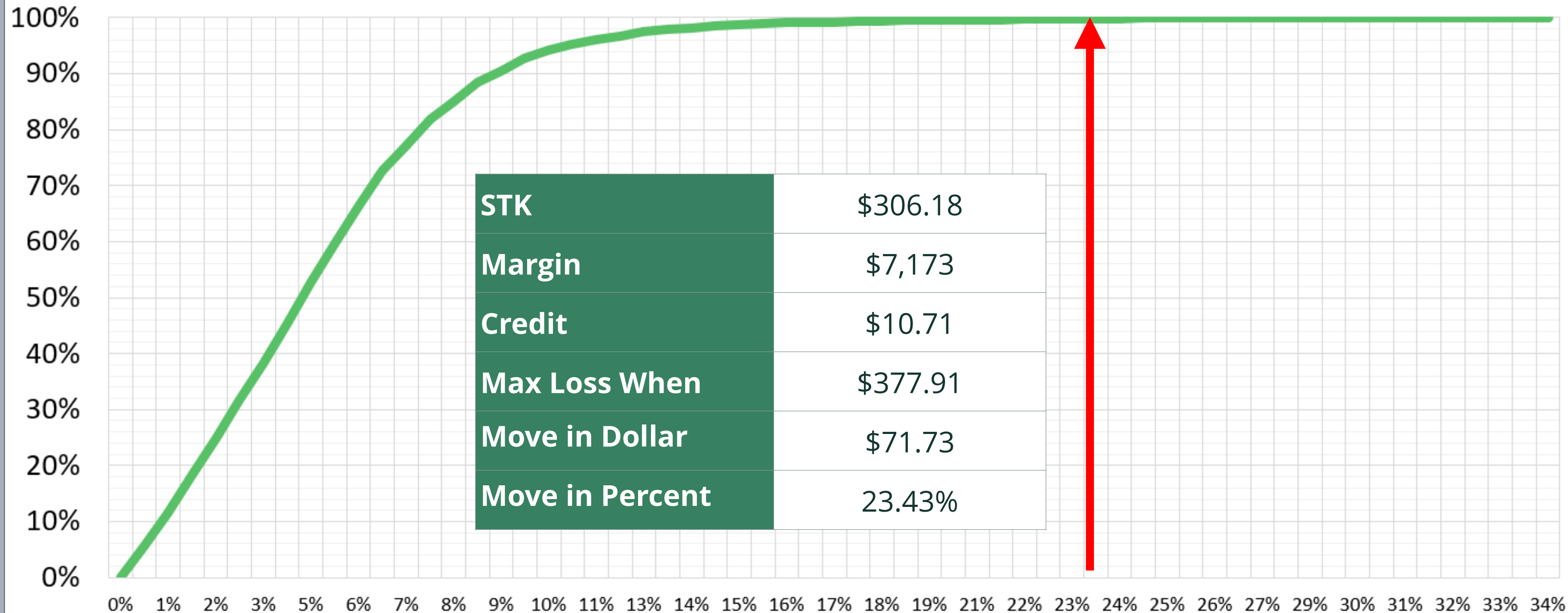
Acc. Percentage for Positive RTN ($QQQ, 39D)
