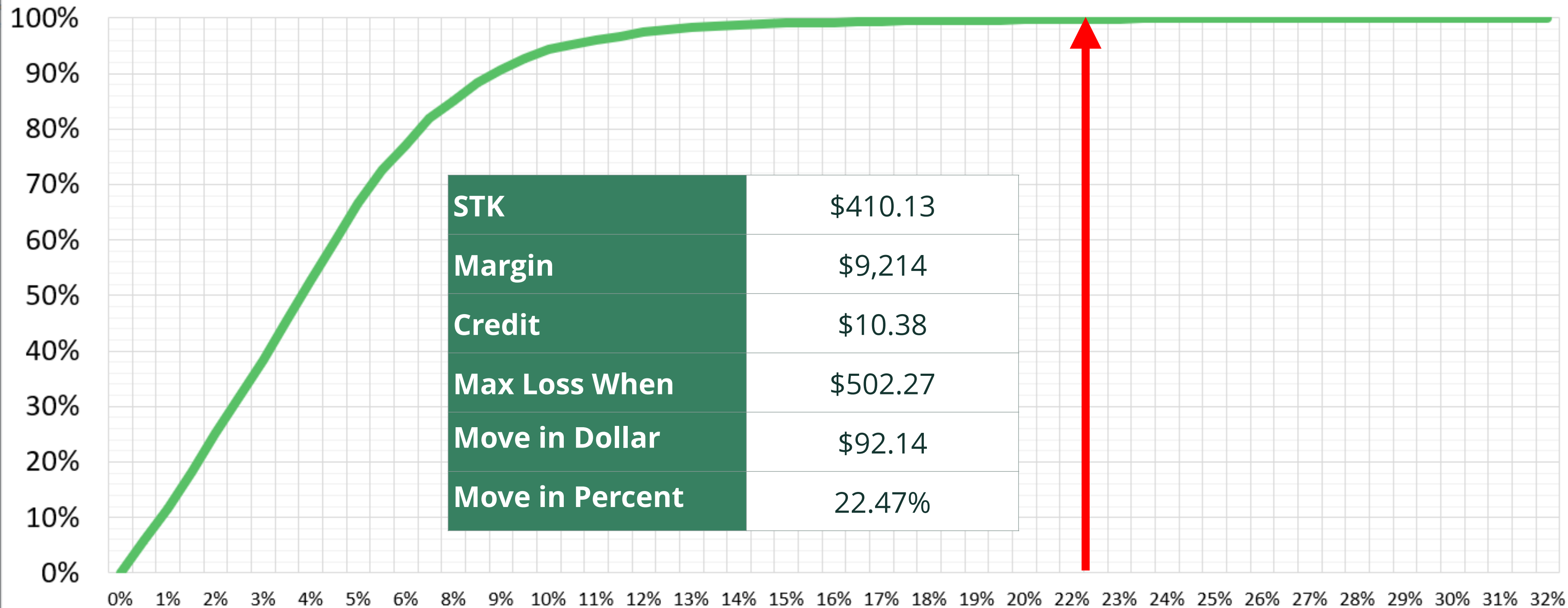
Acc. Percentage for Positive RTN ($SPY, 39D)
