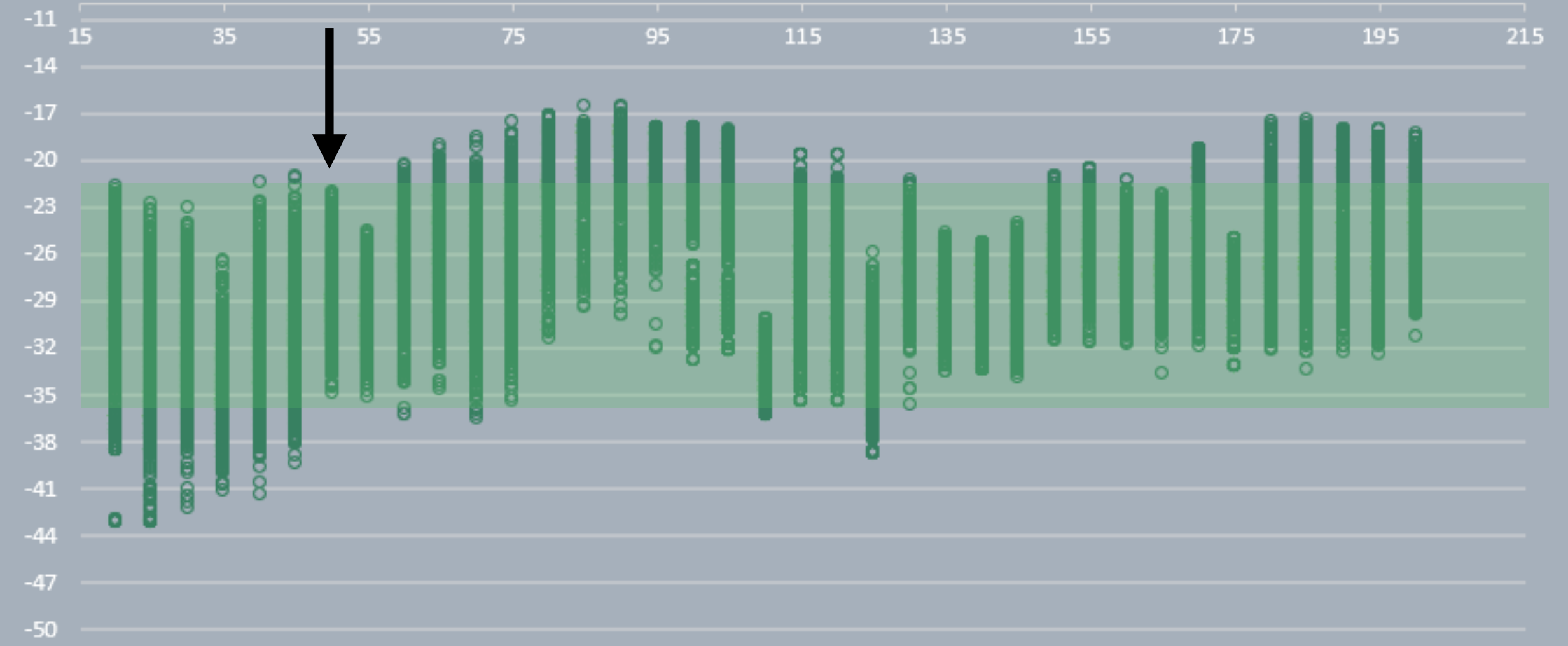
MDD, Overlay SPY Trend, SMA Permutation
